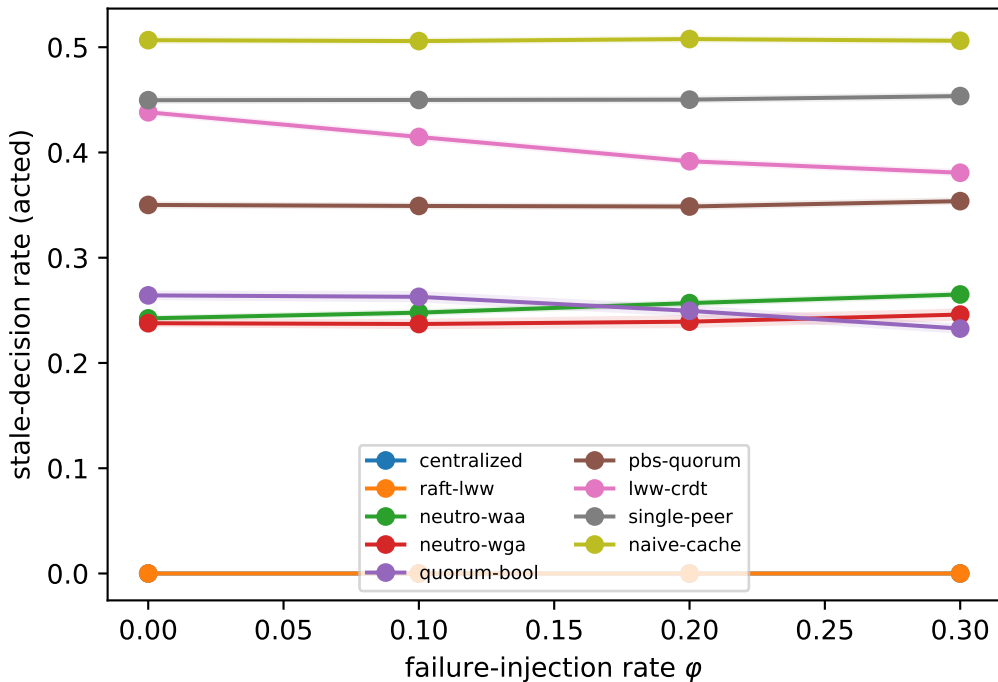
Stale-decision rate vs. failure rate (S2)
