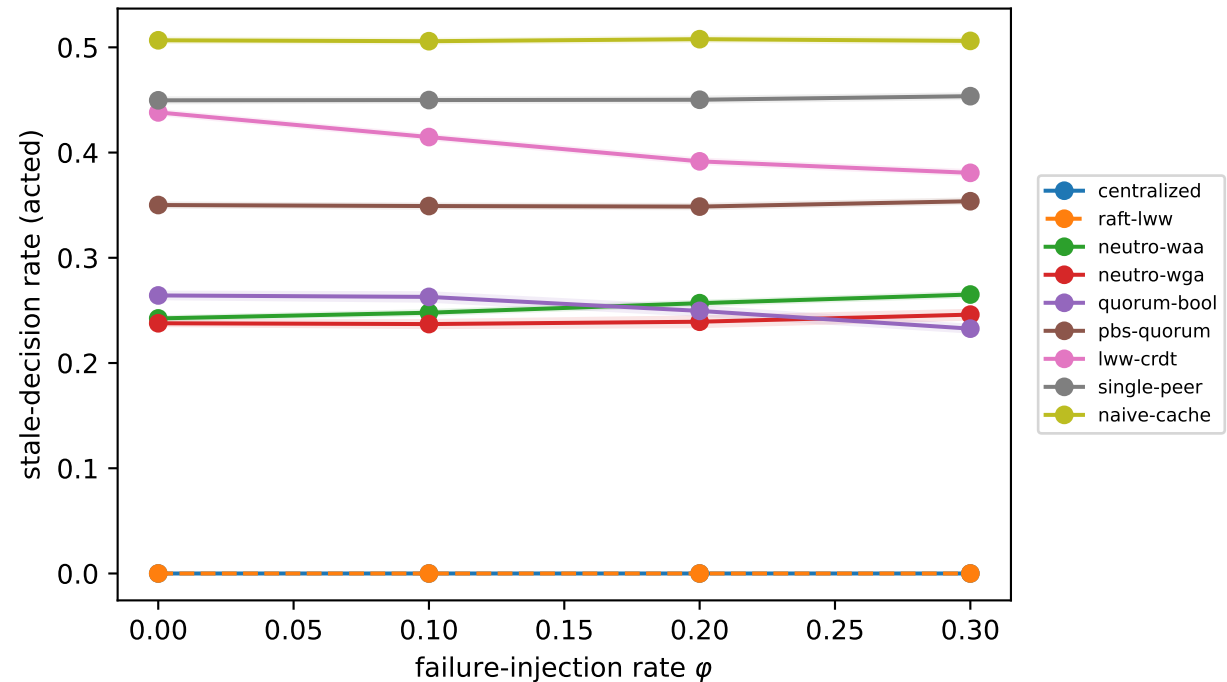
Stale-decision rate vs. failure rate (S2)
