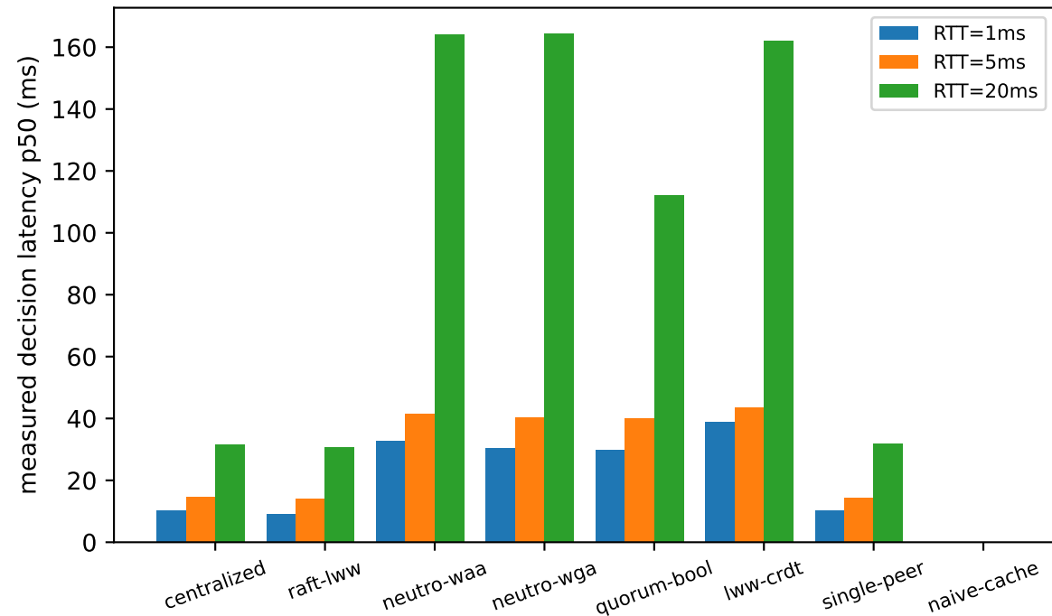
Measured latency on the real HTTP testbed (localhost)
