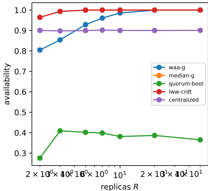
Scalability with cluster size (S2, \phi=0.1 )
