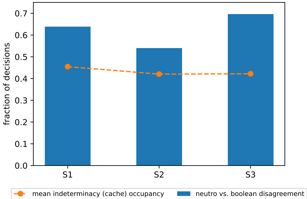
Signal richness of the (T, I, F) axis ( \phi = 0.1 )
