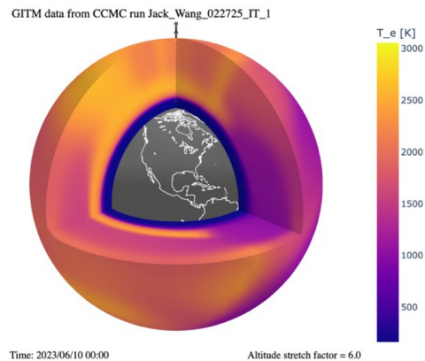
Kamodo plotting of GITM run Jack_Wang_022725_IT_1
