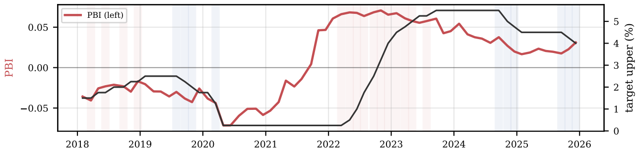
(a) PBI vs. fed funds target
