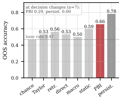
(c) decision accuracy vs. baselines
