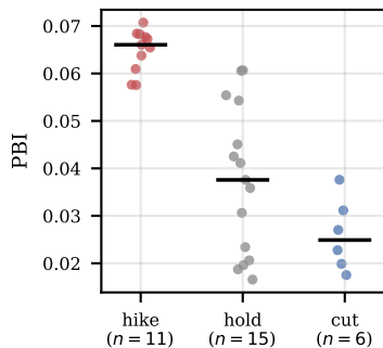
(b) PBI by decision (2022--25)
