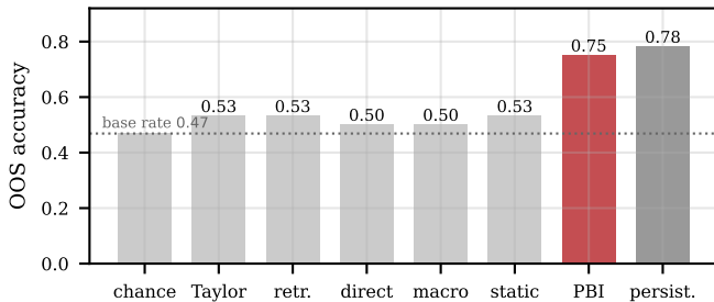
(c) decision accuracy vs. baselines
