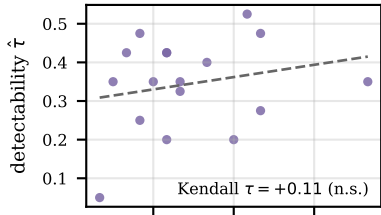
(c) the two axes are uncorrelated
