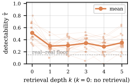
(e) detectability vs k
