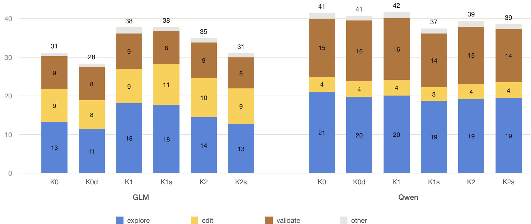
Mean tool calls per acting run [calls]
