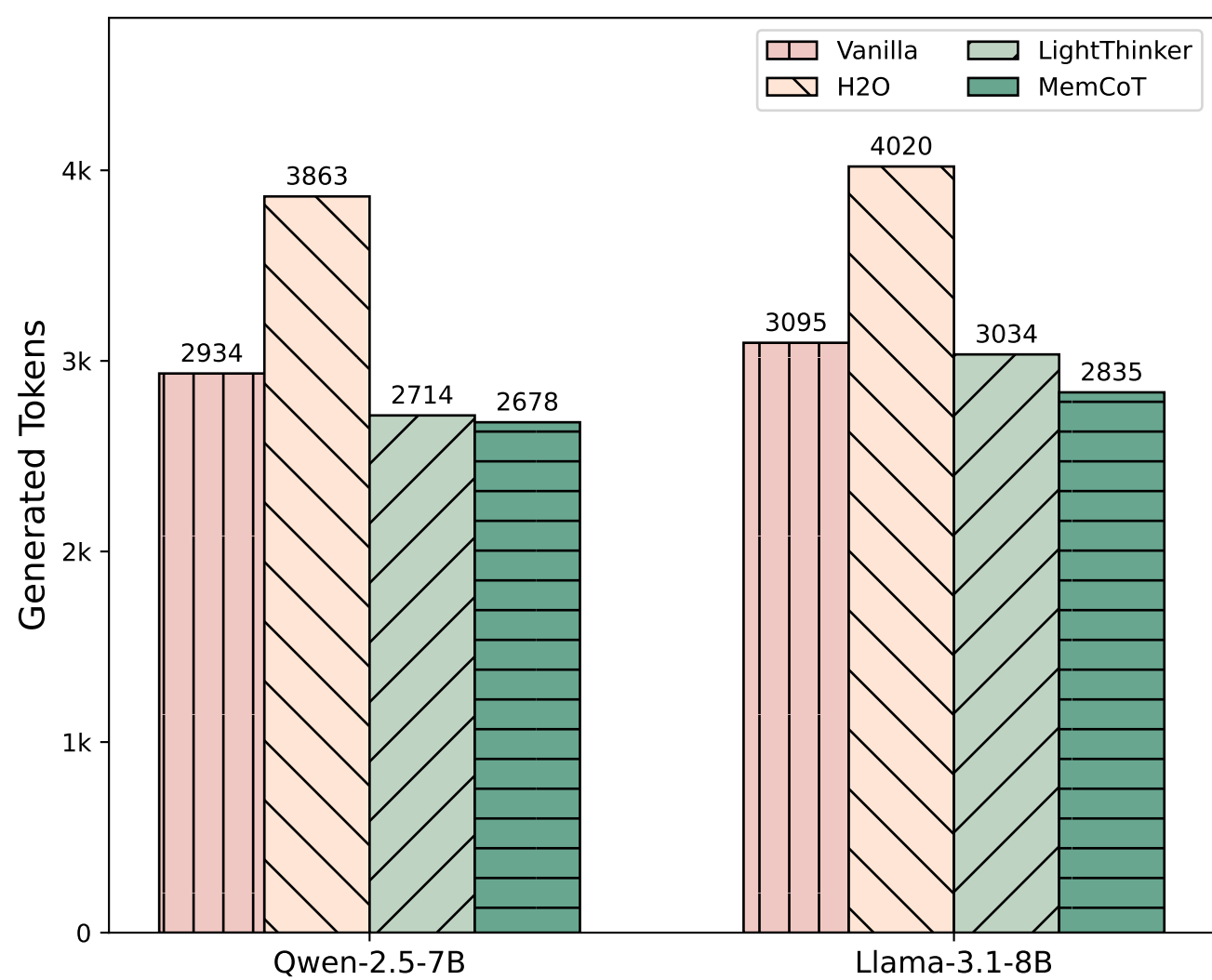
(a) Average number of generated tokens across the four datasets
