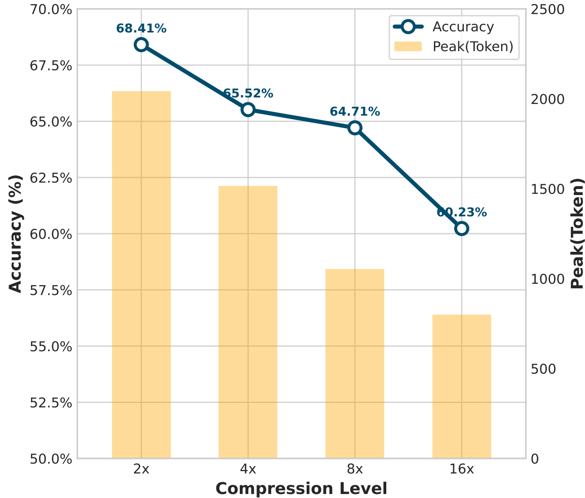
(b) Compression Trade-off
