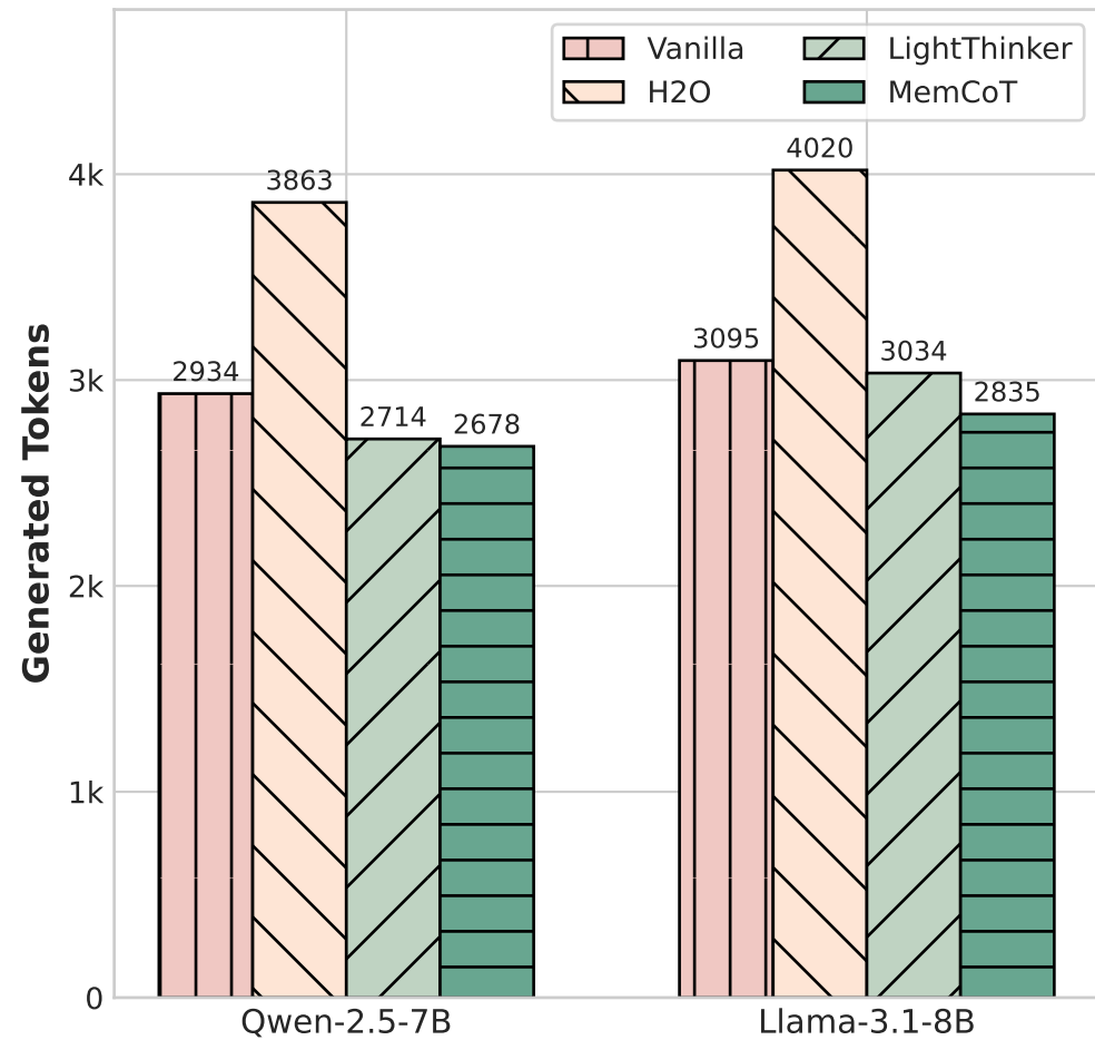
(a) Average Generated Tokens
