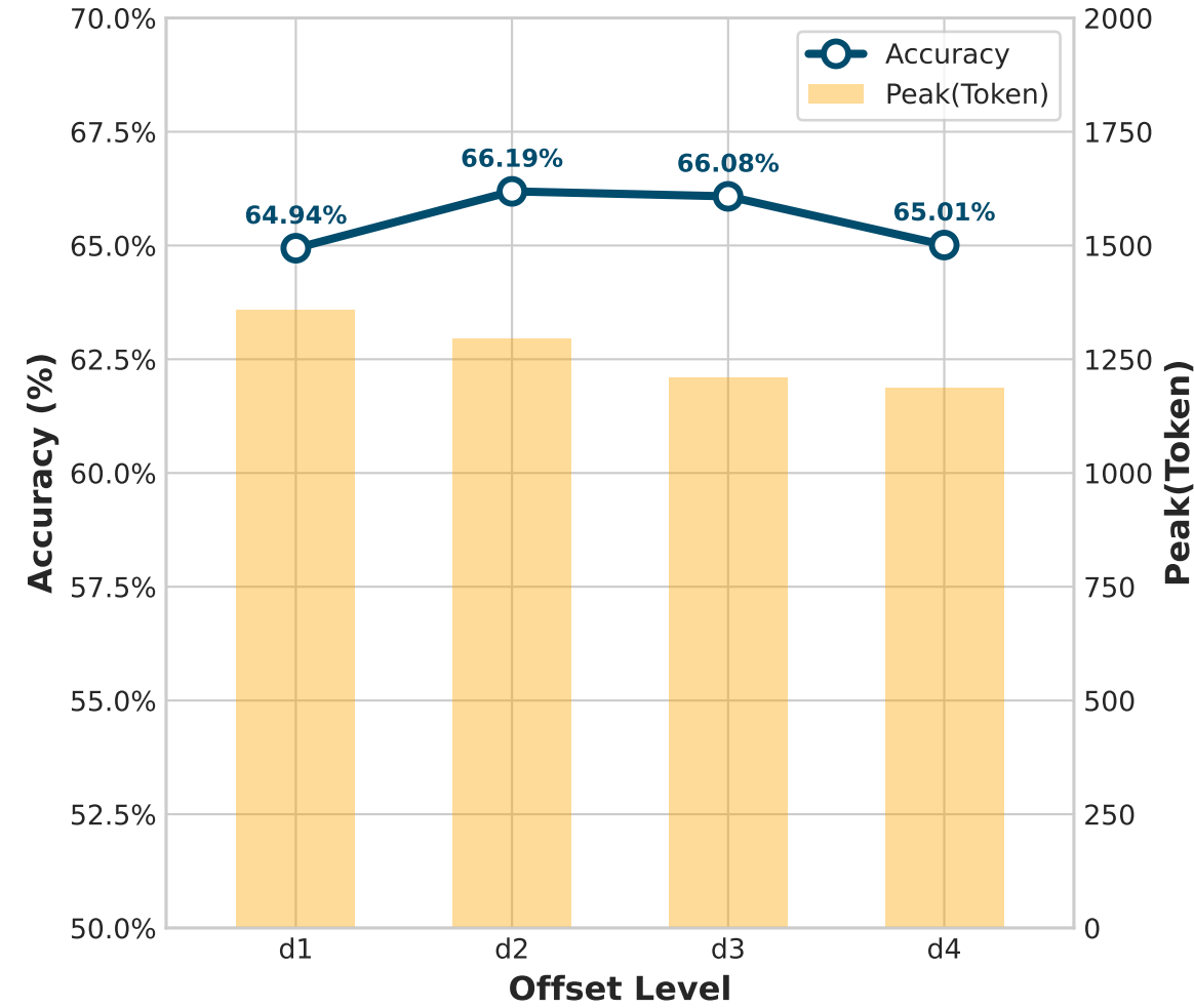
(c) Offset Trade-off
