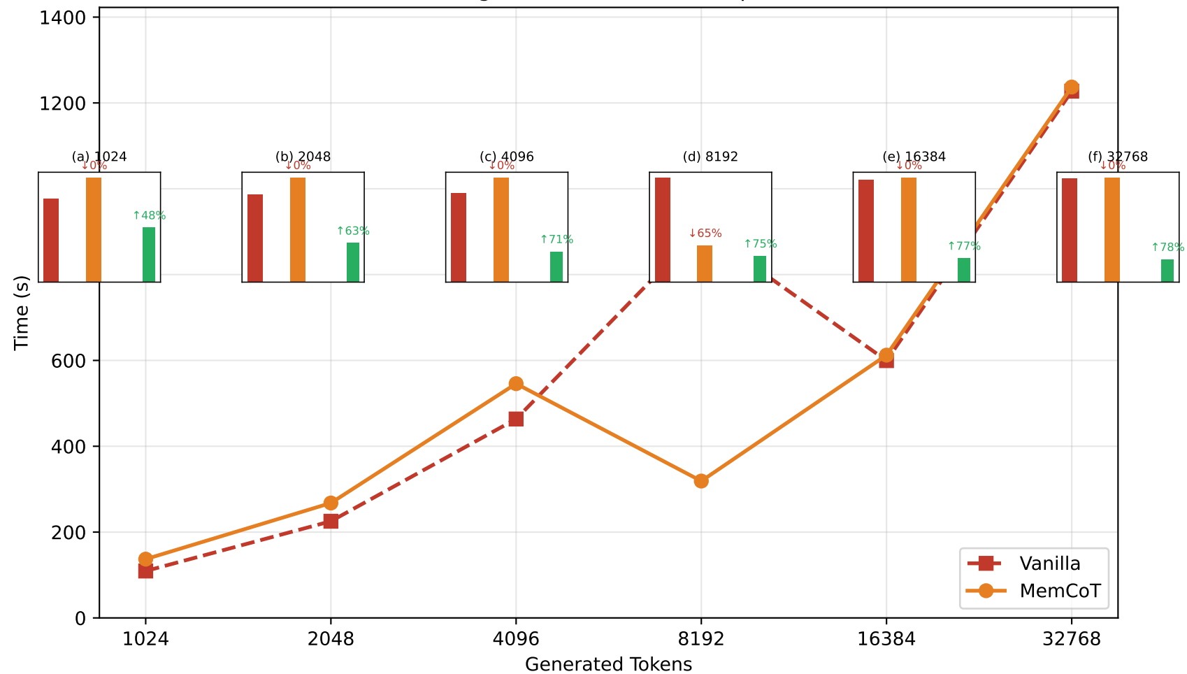
(c) Inference time vs. generated tokens (and peak tokens in insets)
