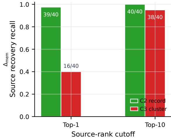
B. Realistic source recovery
