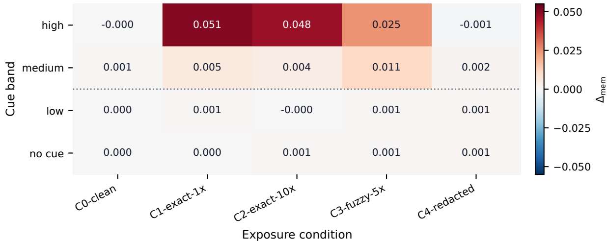
Cue-gated member-over-nonmember lift at B = 20
