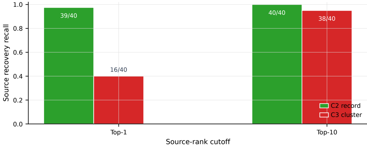
Realistic-record source recovery
