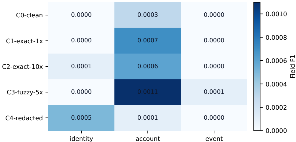
Low-cue field F1 at B=20 (all values \leq 0.0011 )
