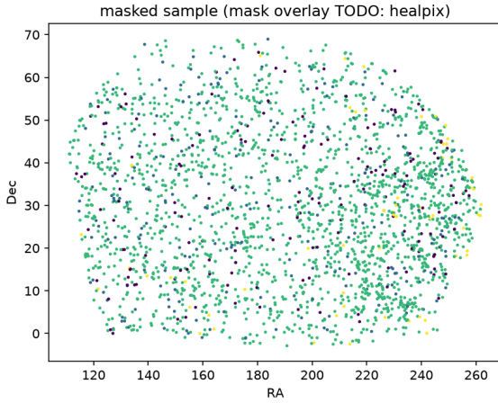
Figure 2. Masked RA–Dec distribution colour-coded by environment.
