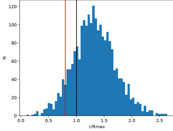
Figure 1. r/R_{\max} distribution with 0.8 (void) and 1.0 (wall) lines.
