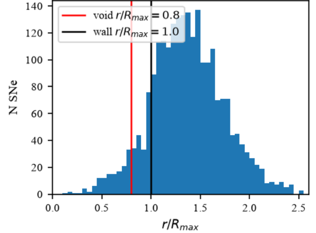
Figure 1. r/R_{\max} for N = 2367 cosmology-grade SNe (void r/R_{\max} < 0.8 , N = 142 ; wall > 1.0 ). Vertical lines mark the analysis thresholds.
