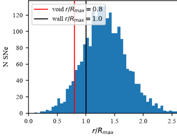
Figure 1. r/R_{\max} for N = 2367 cosmology-grade SNe (void r/R_{\max} < 0.8 , N = 176 ; wall r/R_{\max} > 1.0 ). Vertical lines mark the analysis thresholds.
