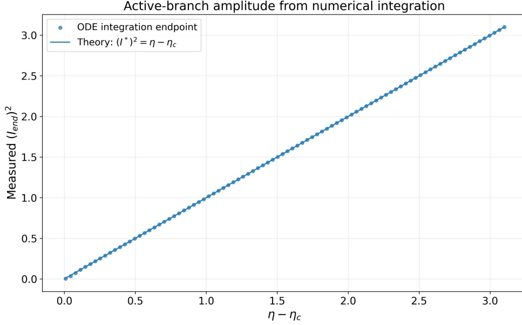
Figure 2: Active-branch amplitude scaling from ODE integration. For fixed \gamma = \xi = \lambda = \beta = 1 , numerical trajectories were integrated from random small initial conditions and allowed to settle. The measured endpoint obeys (I_{\text{end}})^2 \approx \eta - \eta_c , matching the analytic prediction.
