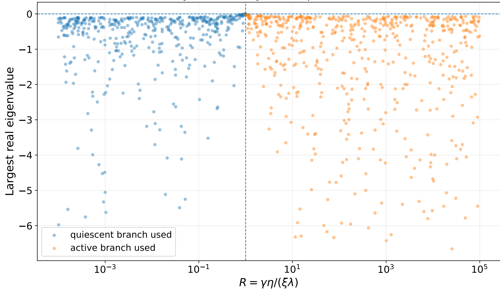
Stability check on synthetic parameter sets
