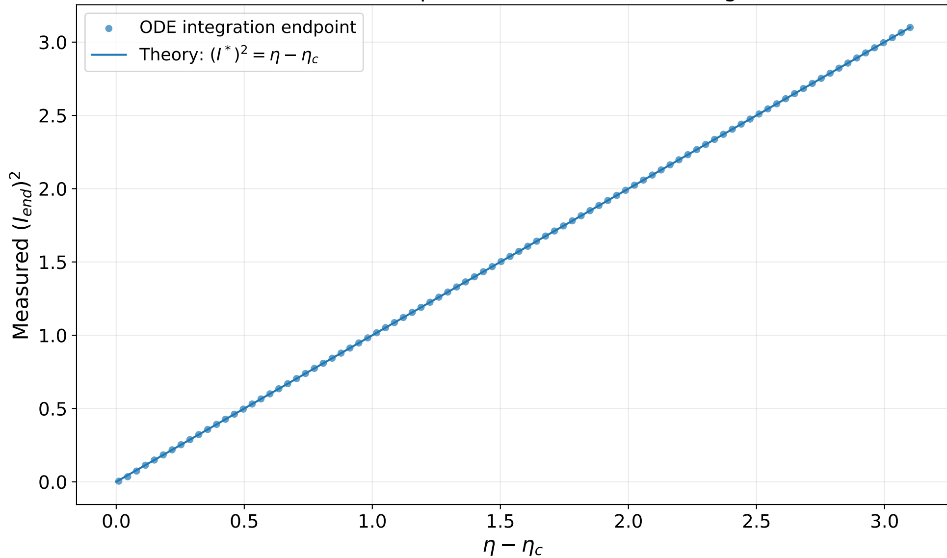
Active-branch amplitude from numerical integration
