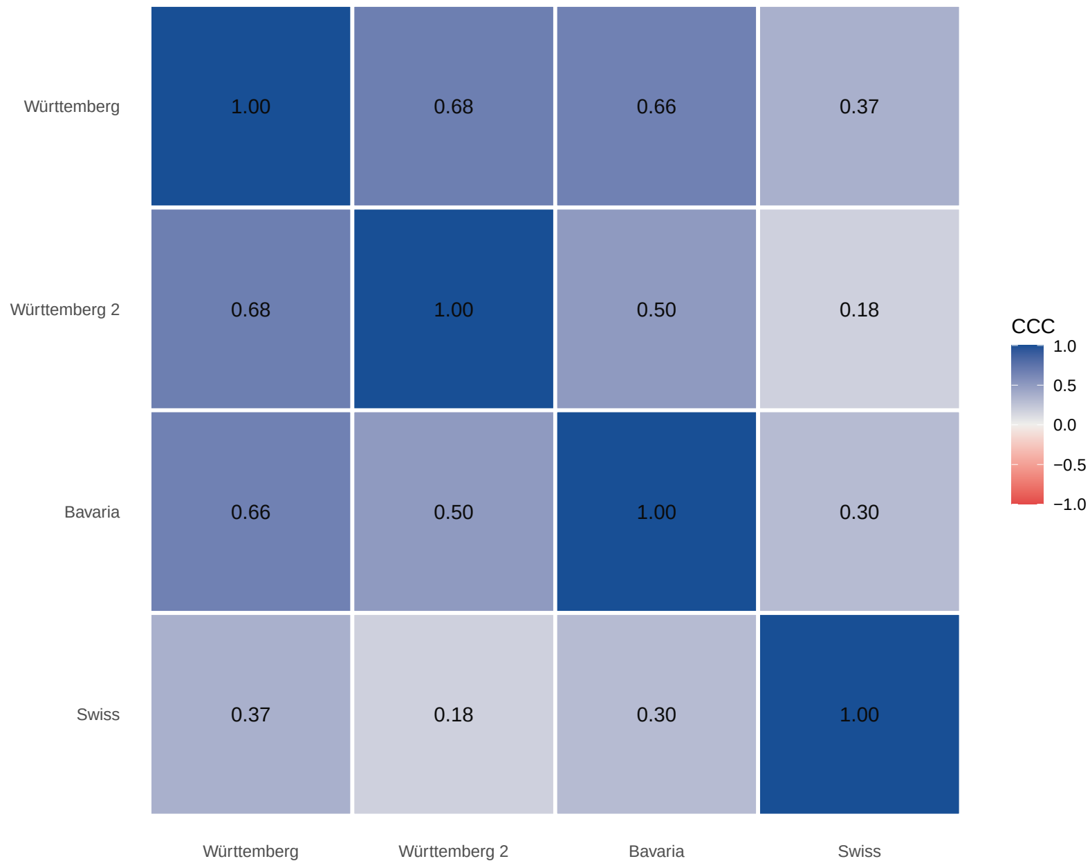
Pairwise CCC – ref_minus_mig (Kst, n=19 shared species)
