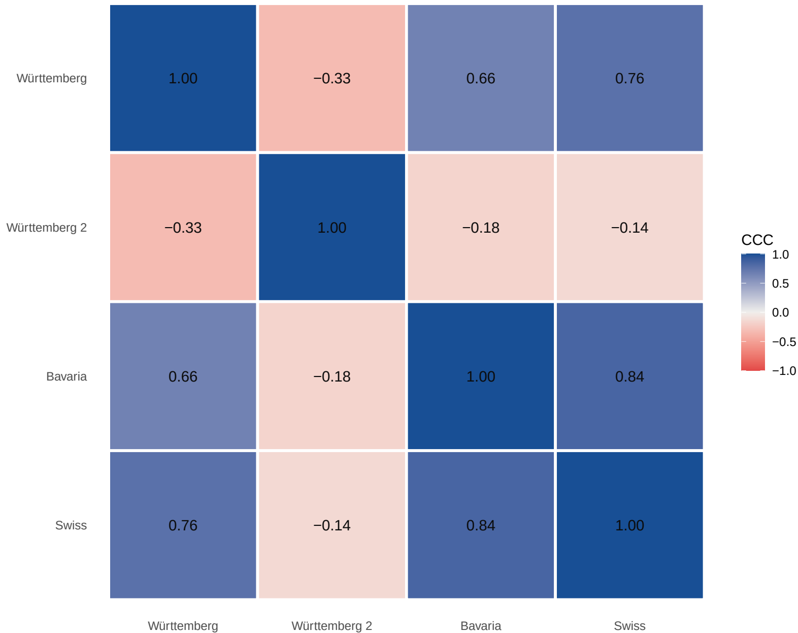
Pairwise CCC – ref_minus_breed (Lst, n=19 shared species)
