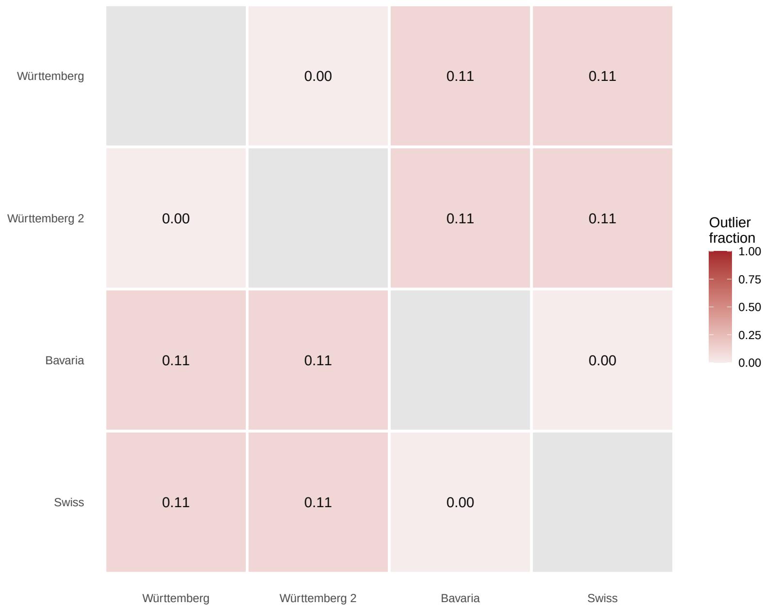
Outlier fraction – ref_minus_breed (Lst, n=19 shared species)
