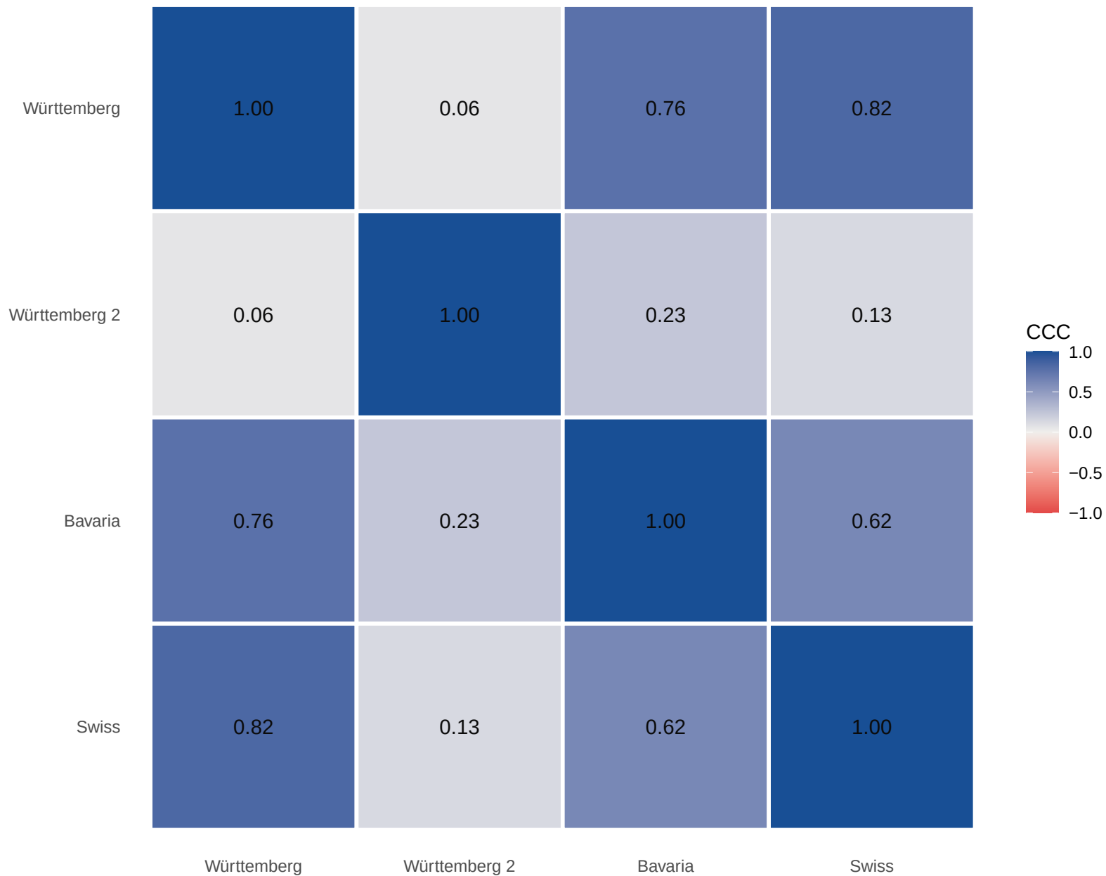
Pairwise CCC – ref_minus_breed (Kst, n=19 shared species)
