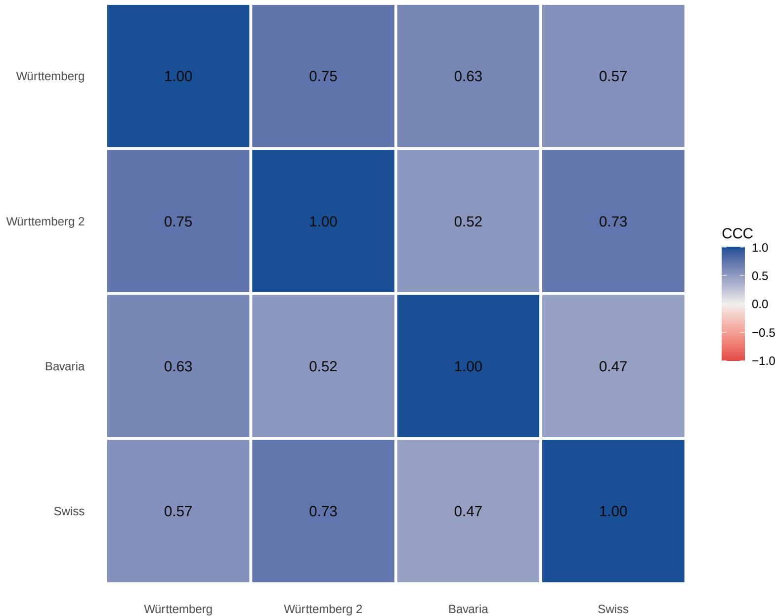
Pairwise CCC – ref_minus_mig (Lst, n=19 shared species)
