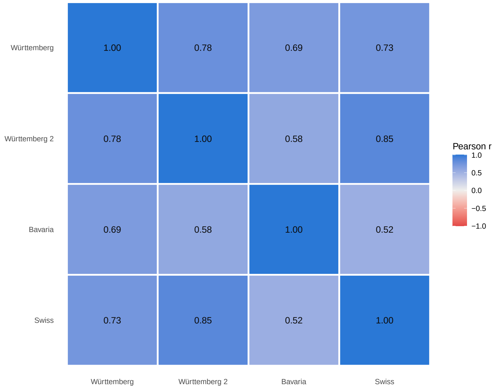
Pairwise Pearson r – ref_minus_mig (Lst, n=19 shared species)
