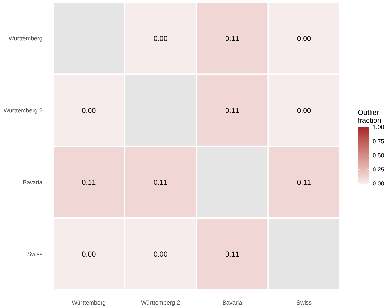
Outlier fraction – ref_minus_mig (Lst, n=19 shared species)
