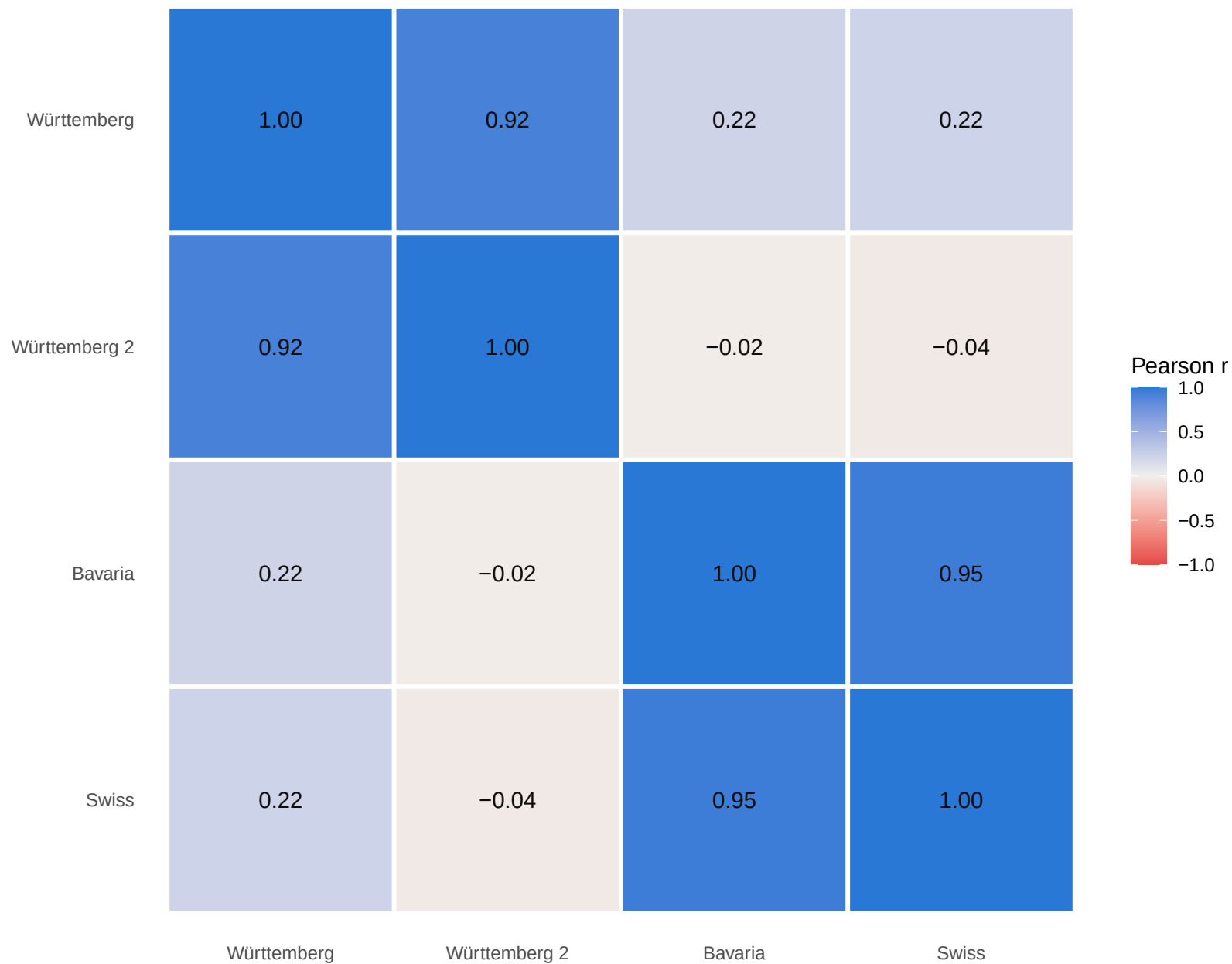
Pairwise Pearson r – ref_minus_breed (Lst, n=19 shared species)
