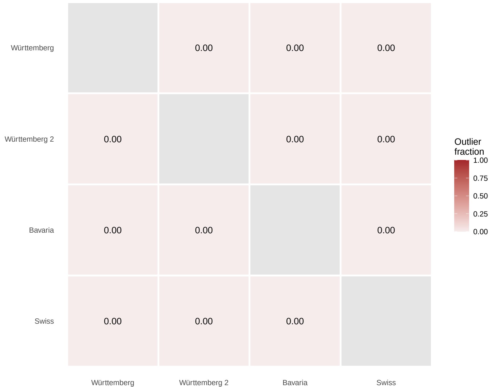
Outlier fraction – ref_minus_breed (Kst, n=19 shared species)
