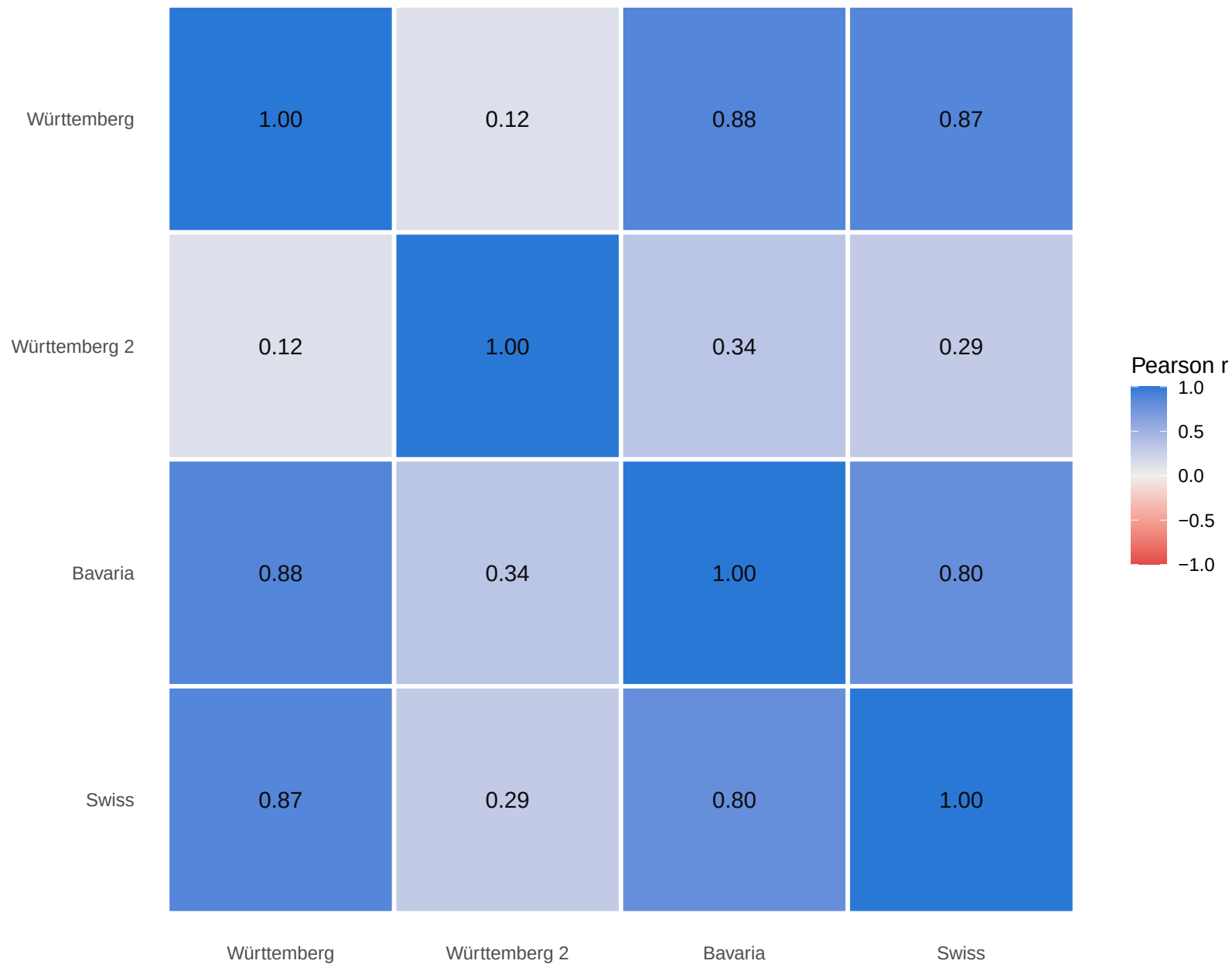
Pairwise Pearson r – ref_minus_breed (Kst, n=19 shared species)
