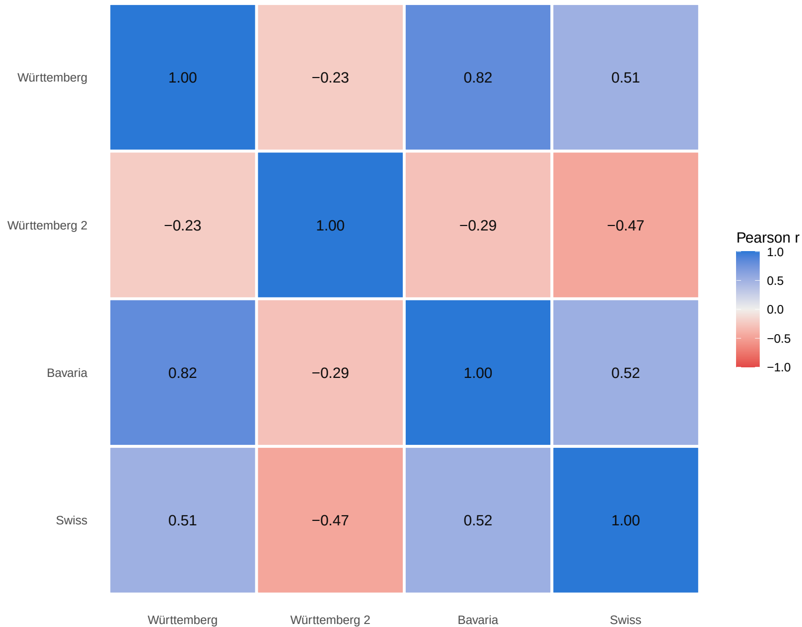
Pairwise Pearson r – ref_minus_mig (Kst, n=19 shared species)
