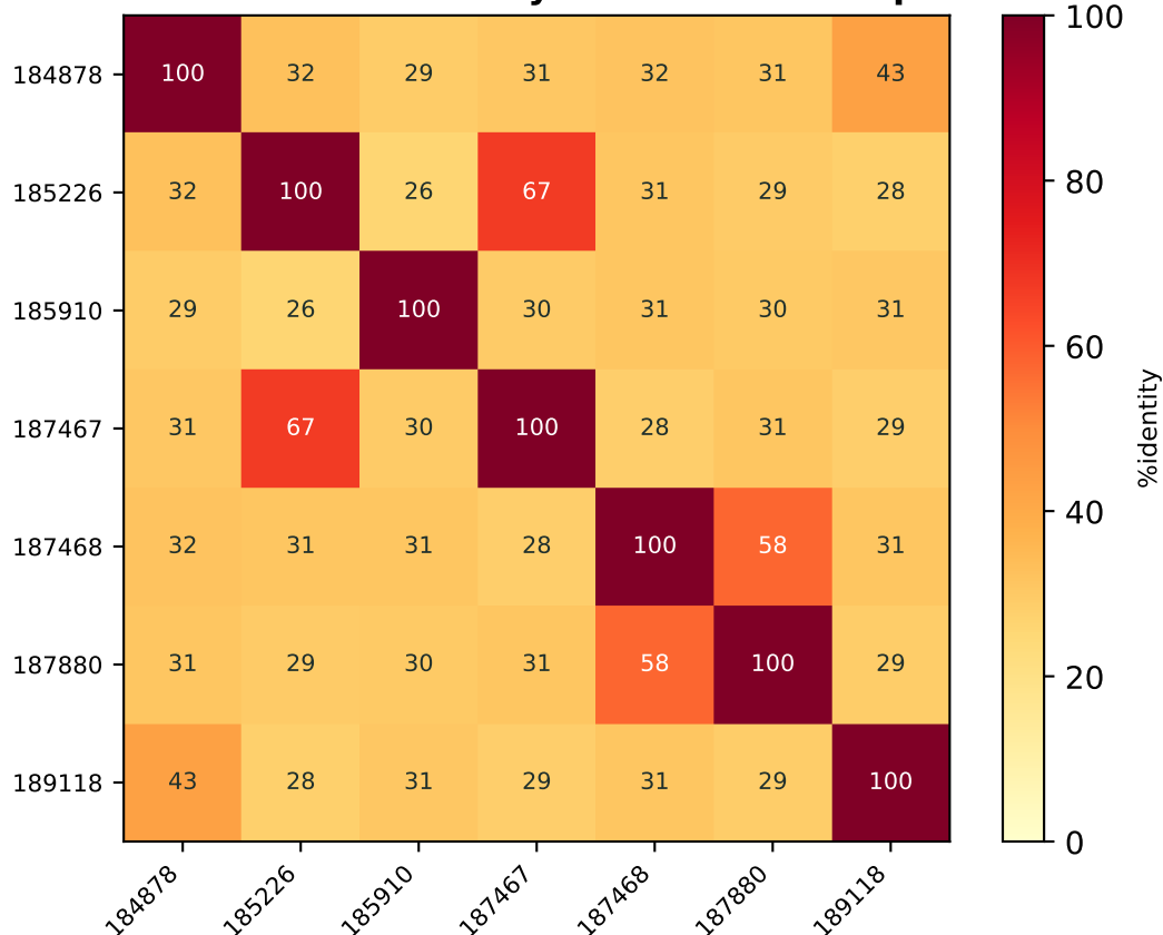
B. Pairwise %identity between all 7 copies
