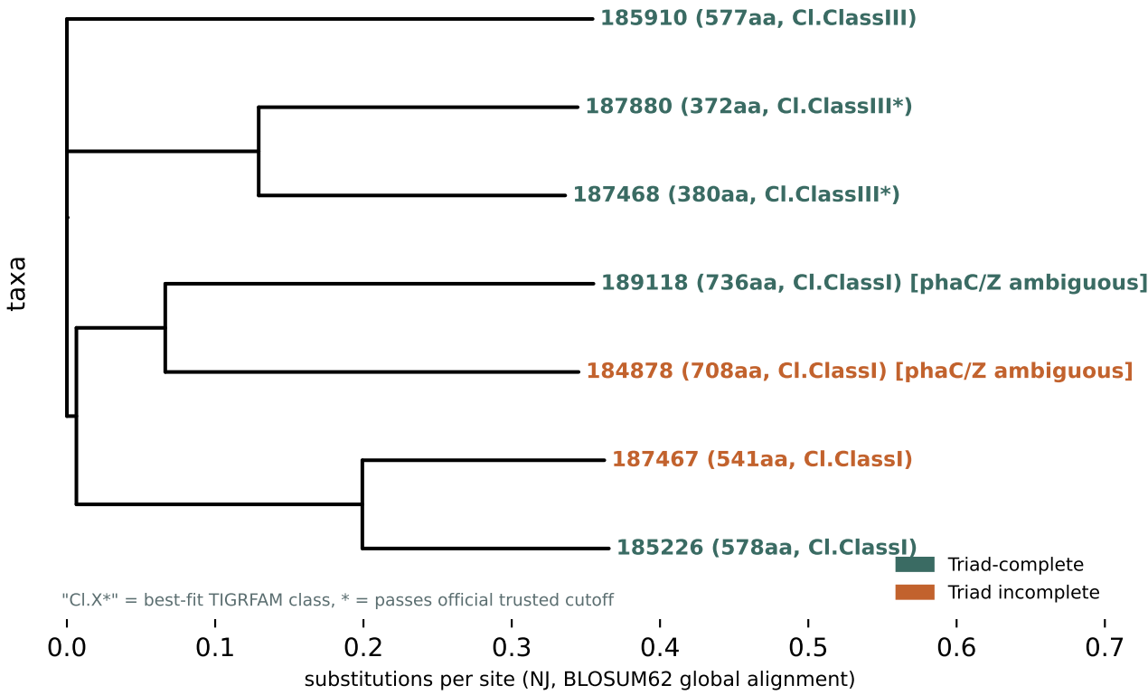
A. Paralog tree: one clade, or independent classes?
