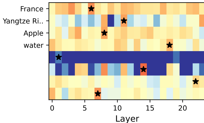
Pythia-1.4B — Attention
