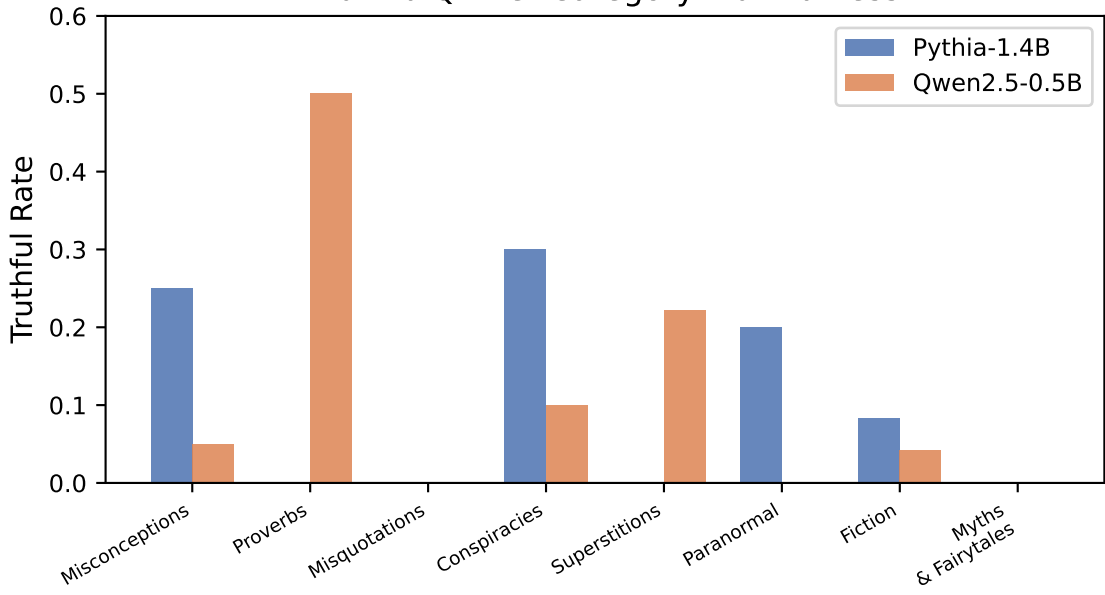
TruthfulQA Per-Category Truthfulness
