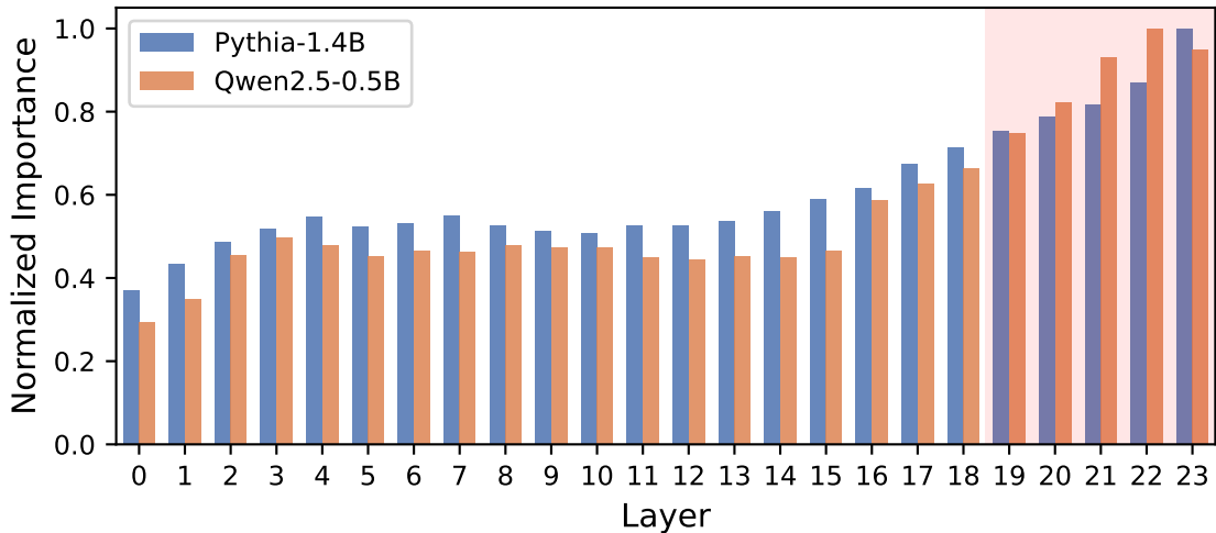
Contrastive Activation Analysis: Layer Importance
