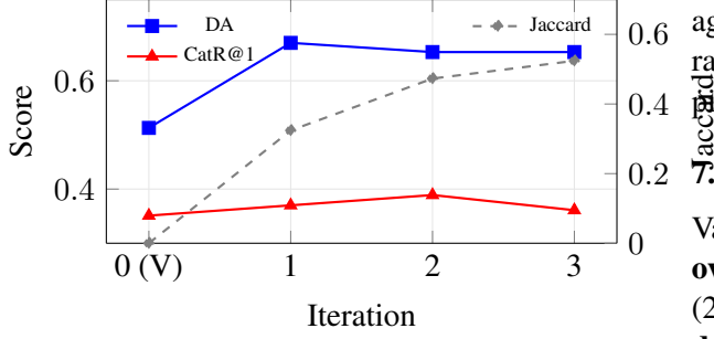
Figure 2: SAD convergence. DA (left axis) converges at Round 1; CatR@1 peaks at Round 2. Hint Jaccard (right axis) rises monotonically, indicating progressive stabilization of the skill vocabulary.
