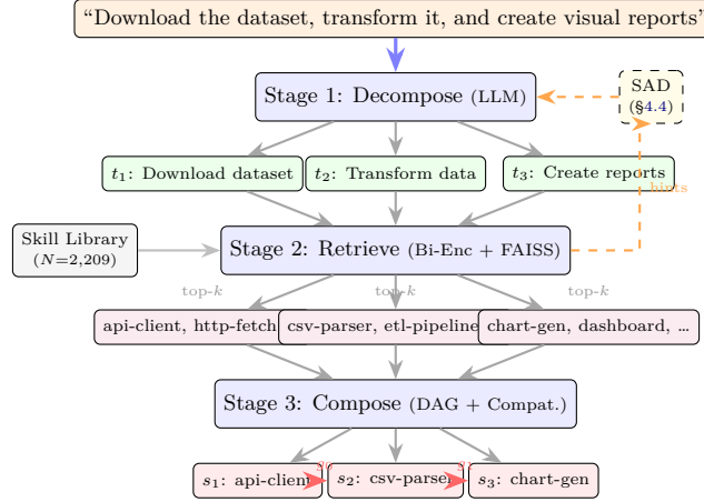
Figure 1: Overview of SkillWeaver. A query is decomposed into sub-tasks, each matched to skills via bi-encoder retrieval, then composed into a DAG. Dashed arrows: SAD feedback loop (§4.4).
