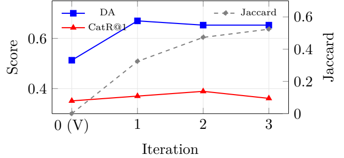
Figure 2: SAD convergence. DA (left axis) converges at Round 1; CatR@1 peaks at Round 2. Hint Jaccard (right axis) rises monotonically, indicating progressive stabilization of the skill vocabulary.
