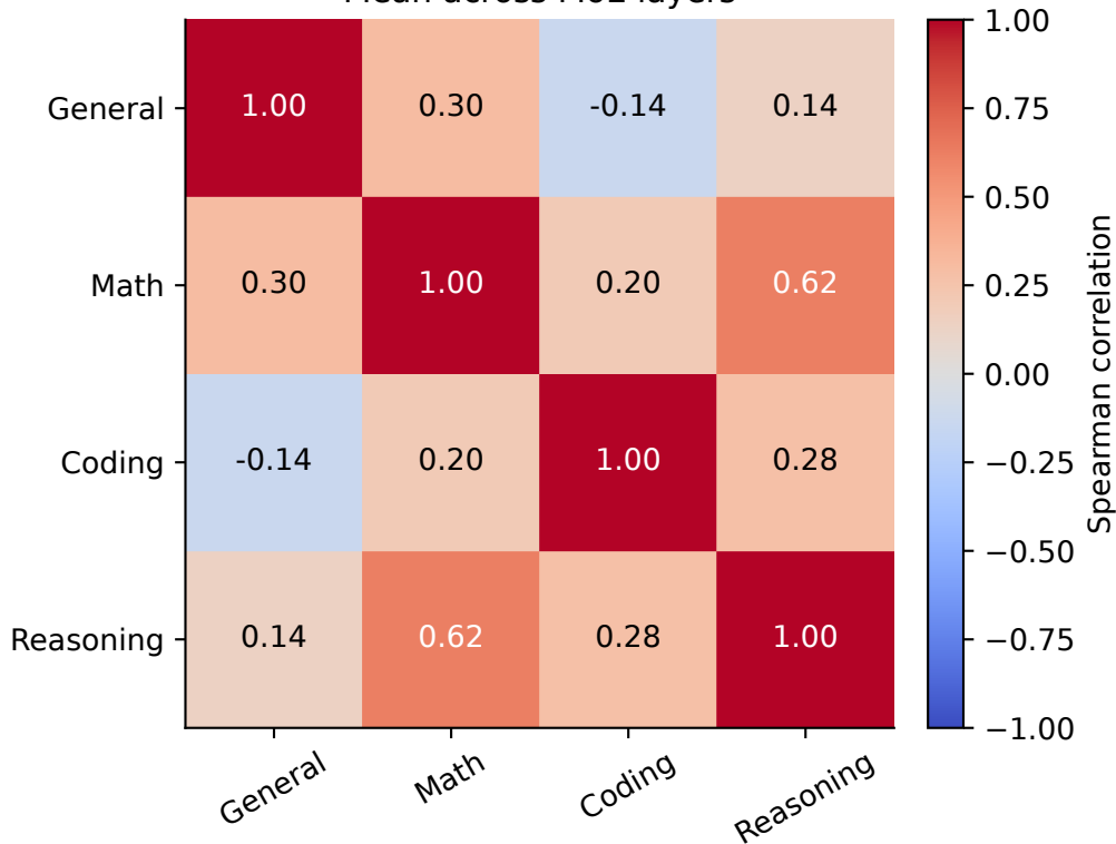
Cross-domain Spearman: Routing frequency Mean across MoE layers
