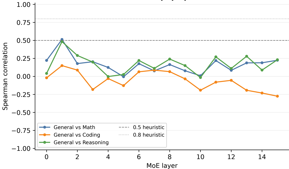
Cross-domain stability by layer: Gate mass
