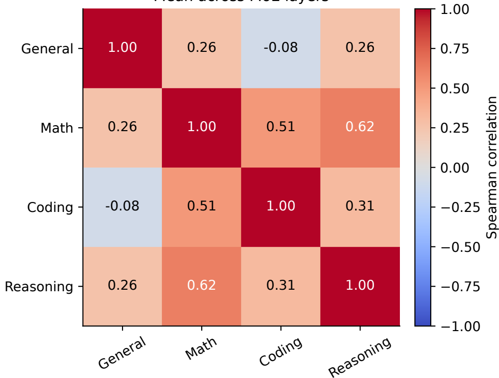
Cross-domain Spearman: Functional contribution Mean across MoE layers
