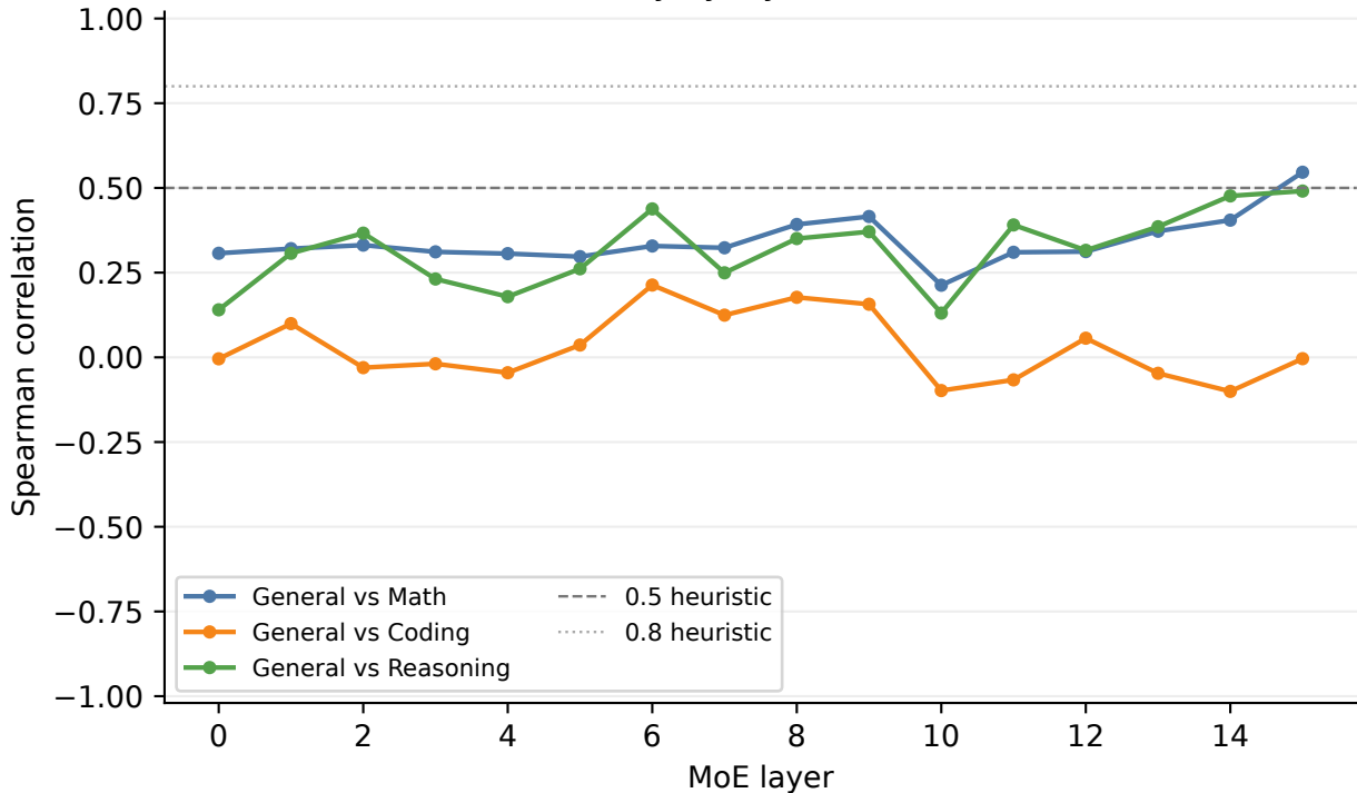
Cross-domain stability by layer: Functional contribution
