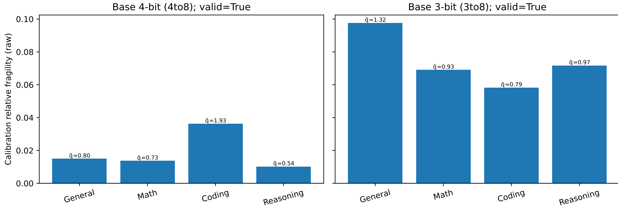
Figure 1: Calibration domain fragility
