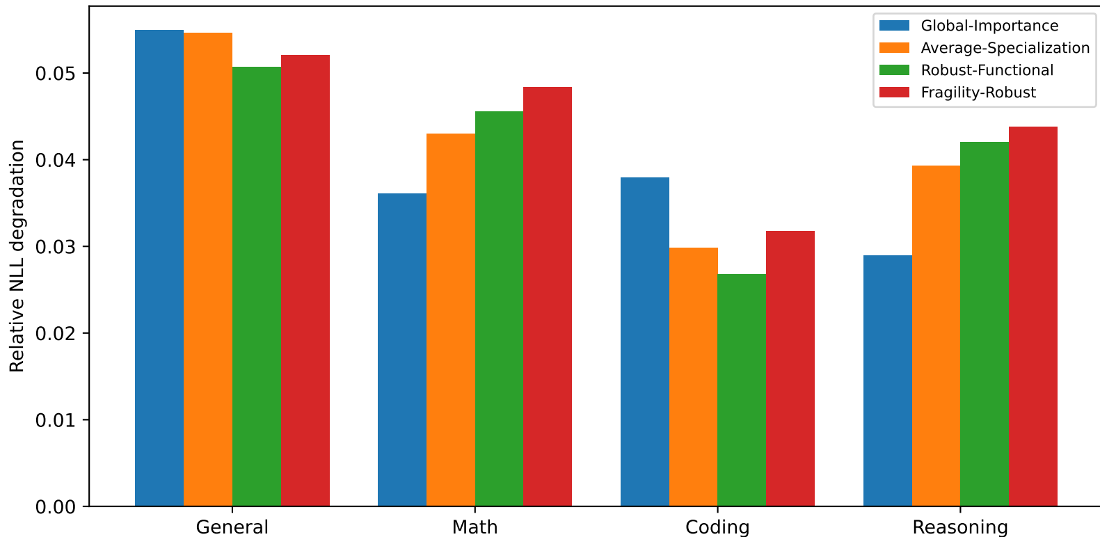
Figure 4: Domain degradation at 20% budget (3to8, development)
