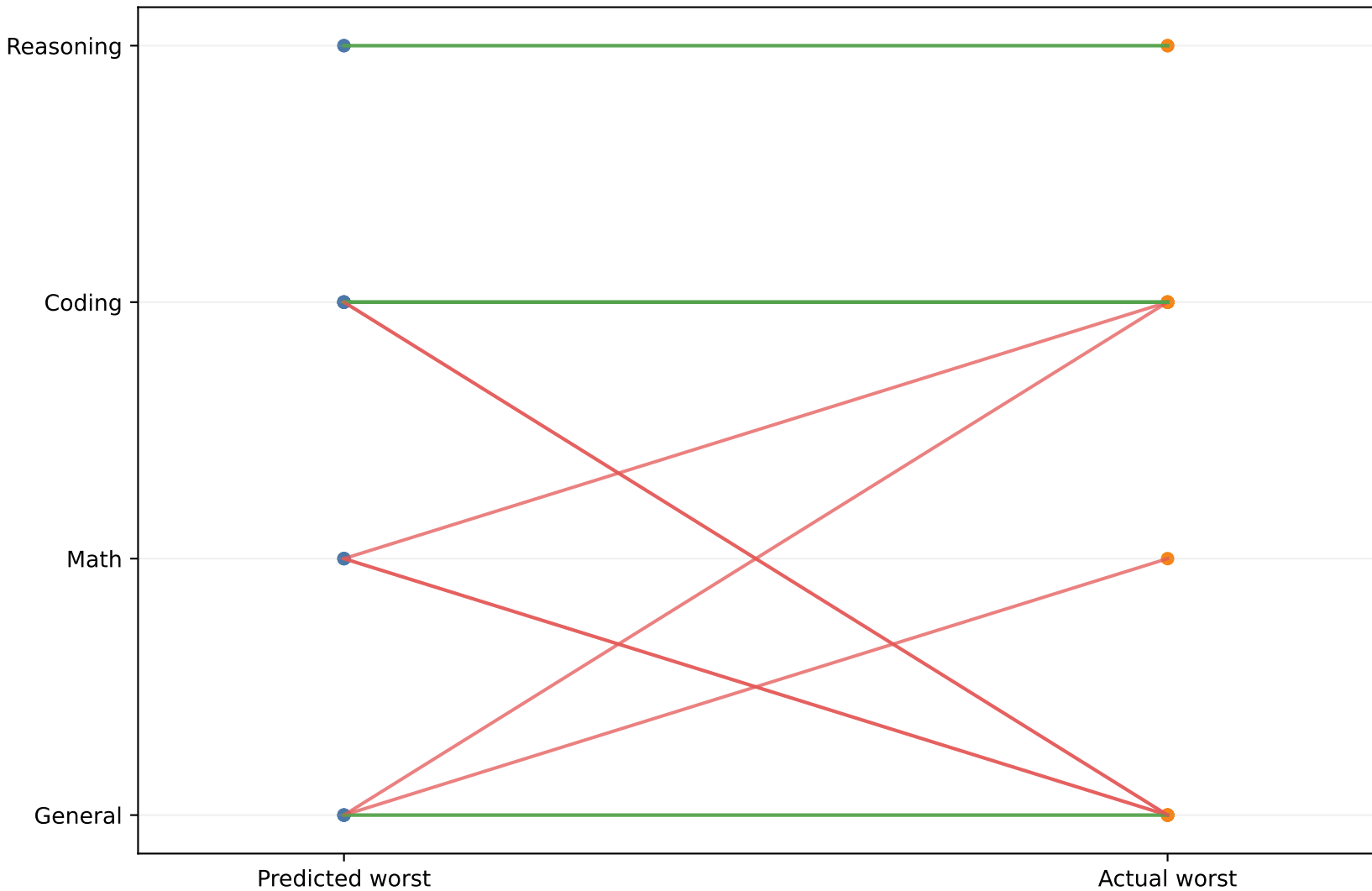
Worst-domain identification for each pilot expert
