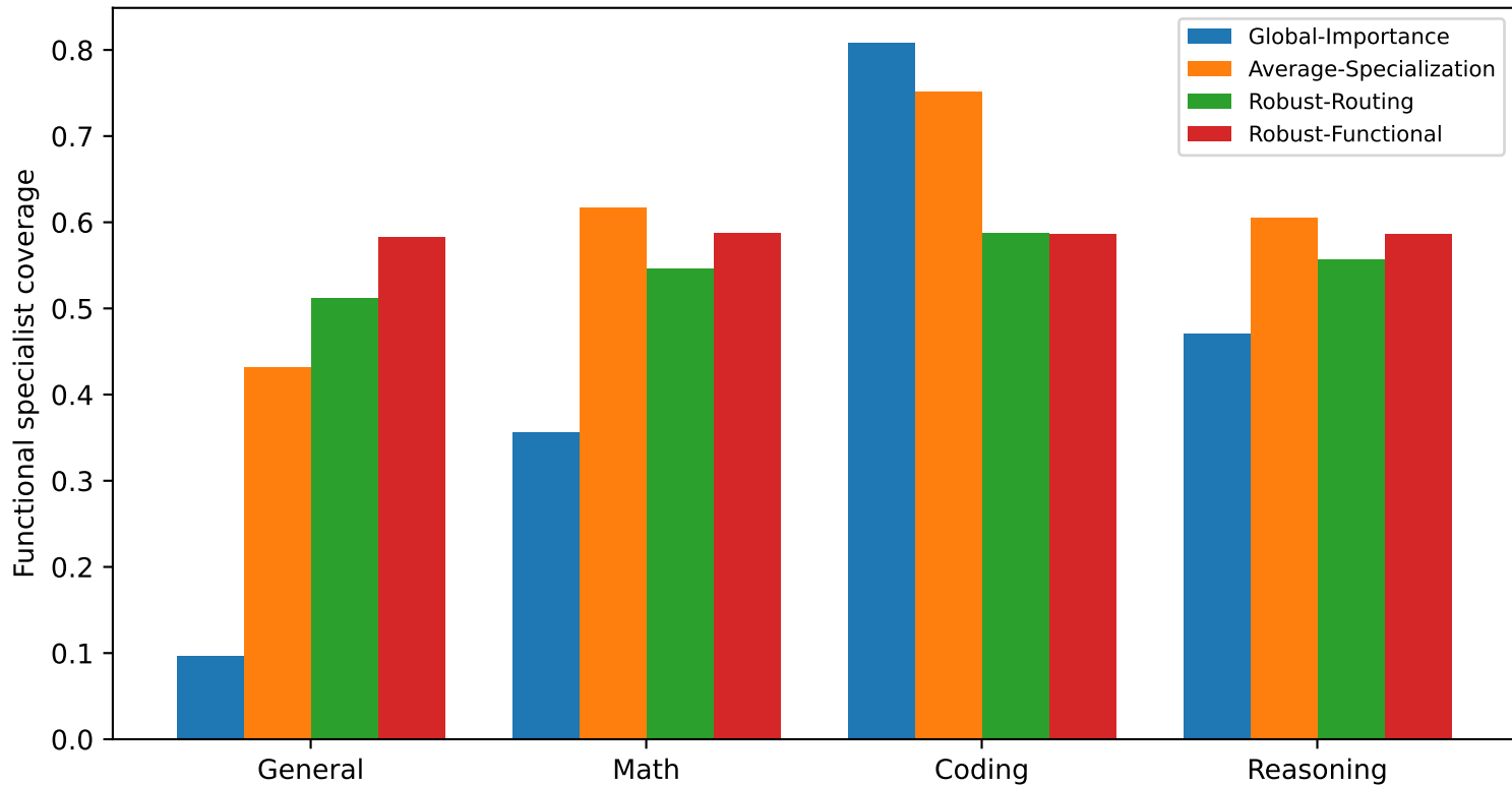
Specialist coverage at 20% budget (4to8)
