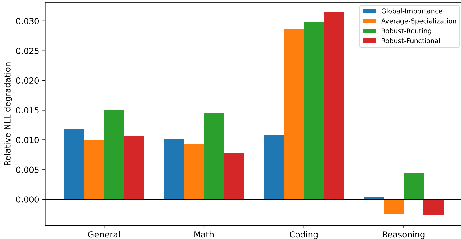
Domain degradation at 20% budget (4to8)
