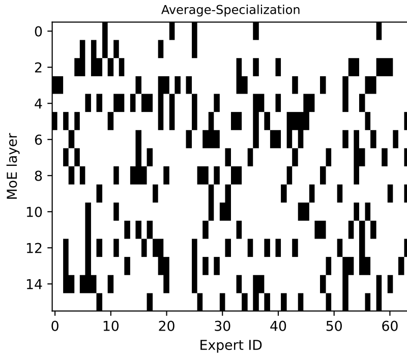
Protected experts at 20% budget (4to8)
