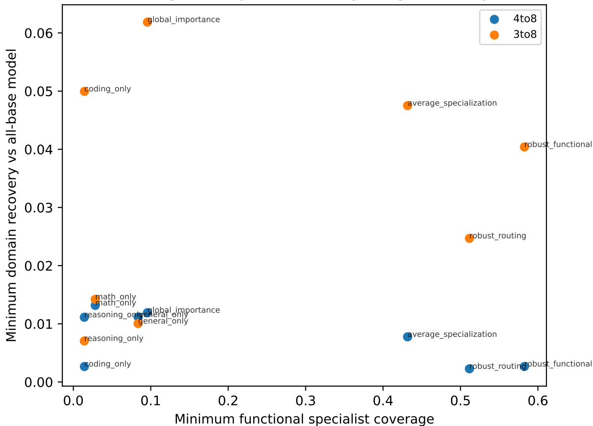
Coverage vs empirical recovery (diagnostic only)
