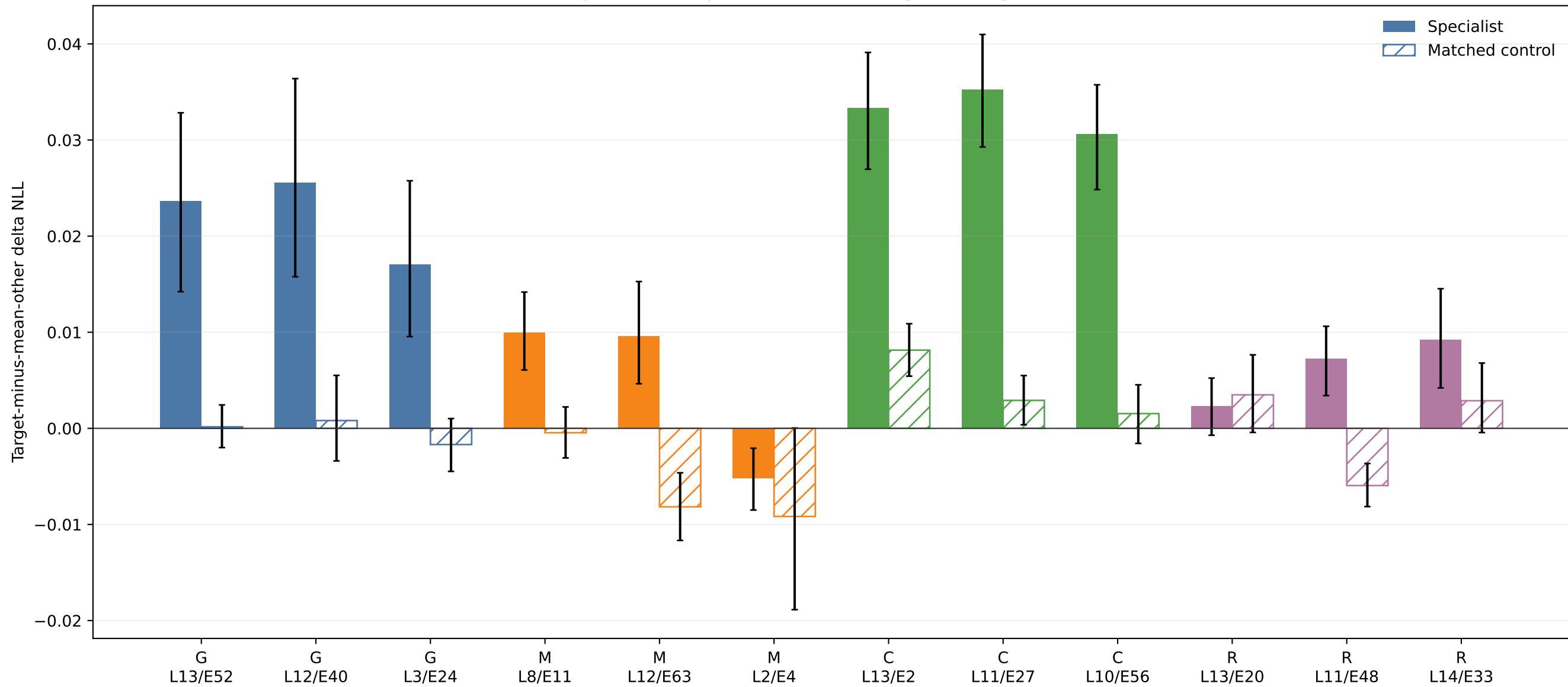
Specialized experts versus same-layer routing controls
