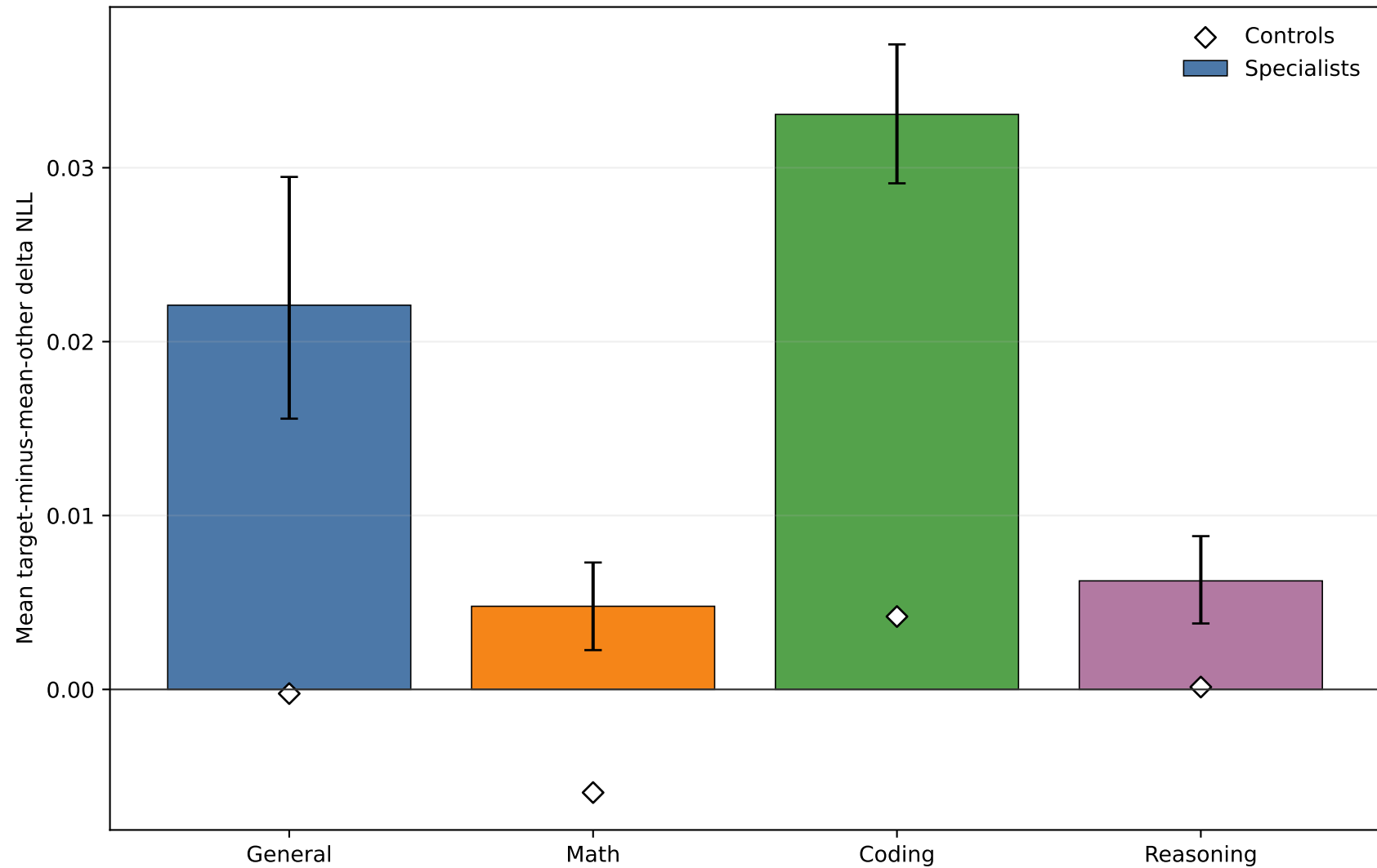
Aggregate causal specificity by target domain
