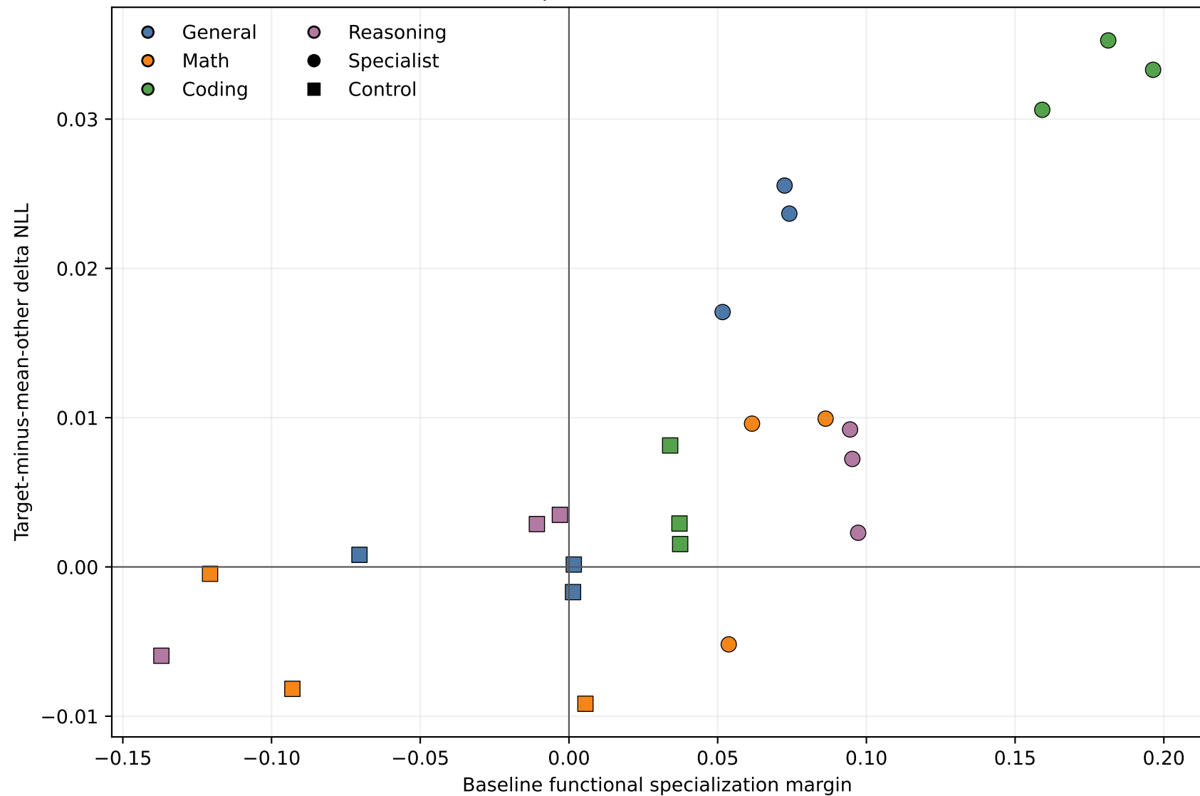
Functional specialization versus causal sensitivity Spearman rho = 0.753
