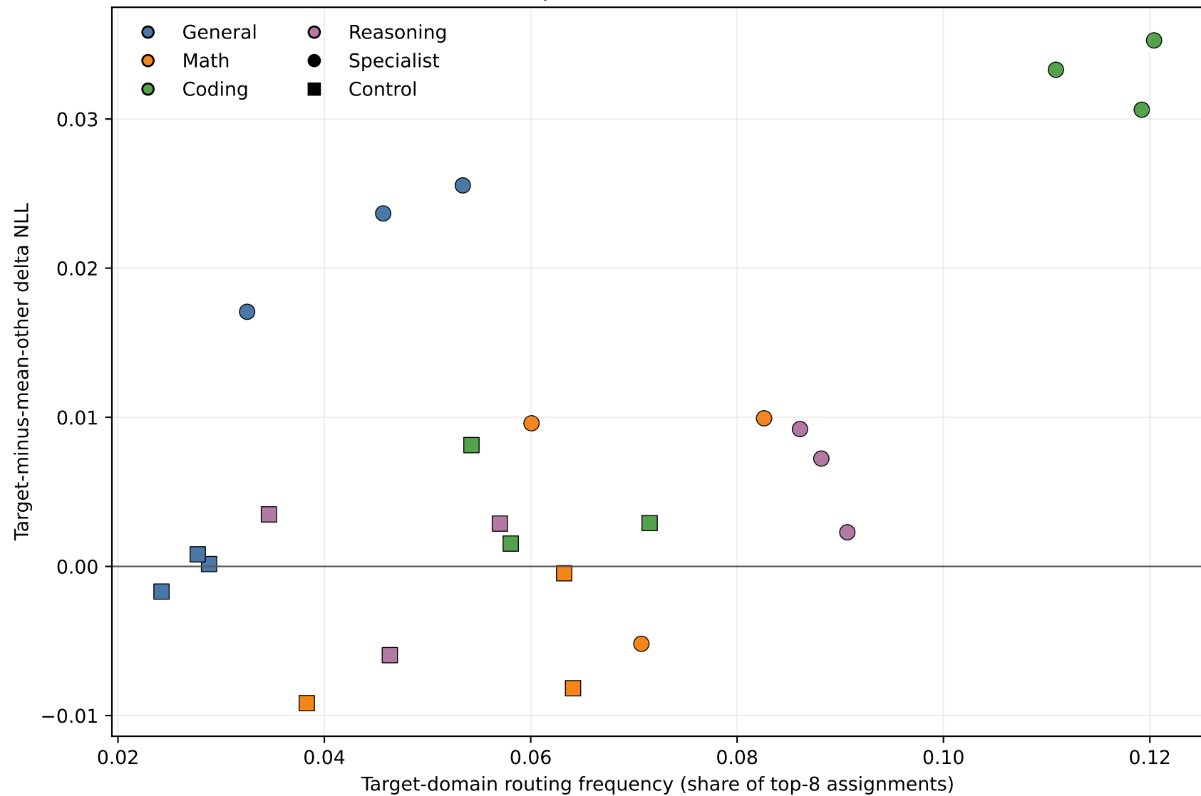
Routing frequency versus causal specificity Spearman rho = 0.417
