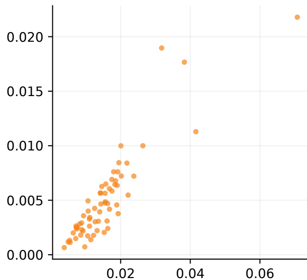
Math, layer 8 Spearman = 0.96
