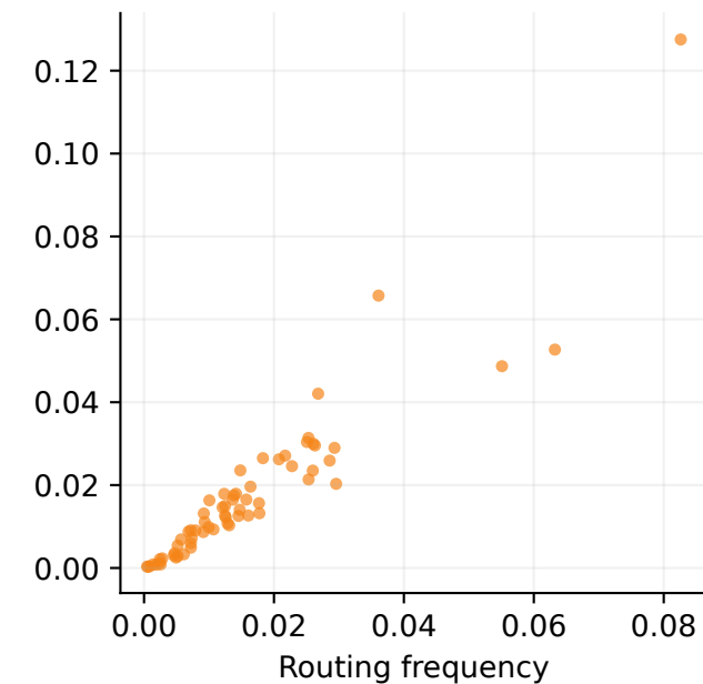
Math, layer 8 Spearman = 0.96
