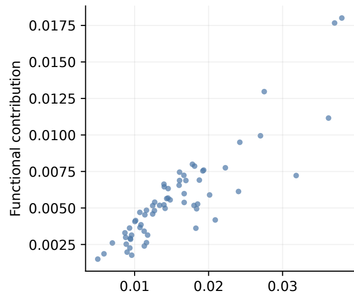
General, layer 8 Spearman = 0.95
