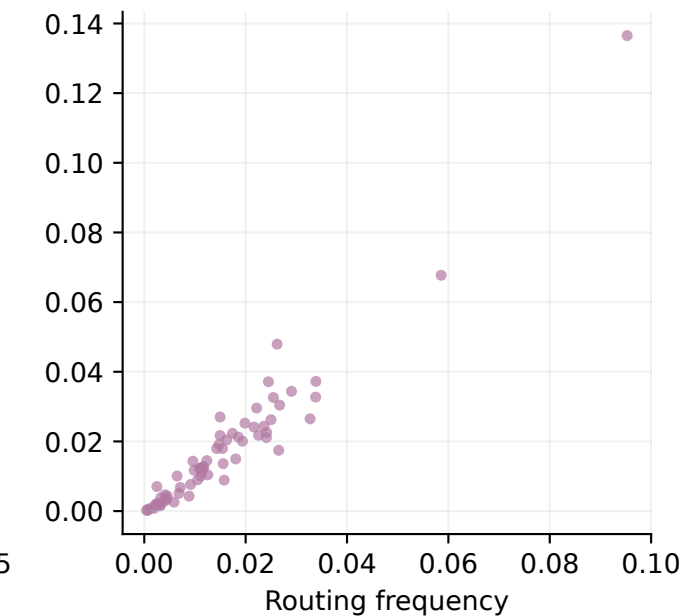
Reasoning, layer 8 Spearman = 0.95
