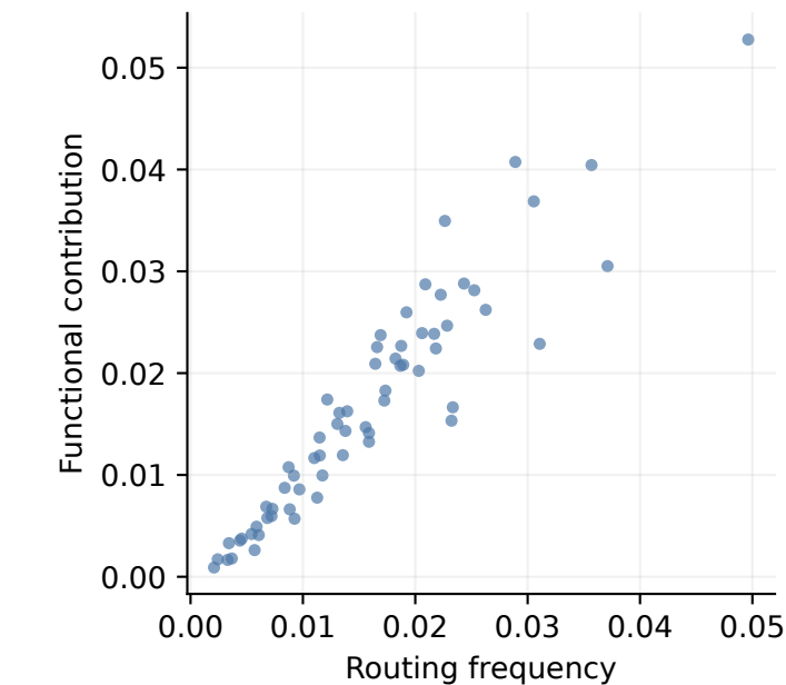
General, layer 8 Spearman = 0.95
