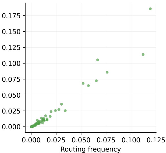
Coding, layer 8 Spearman = 0.98
