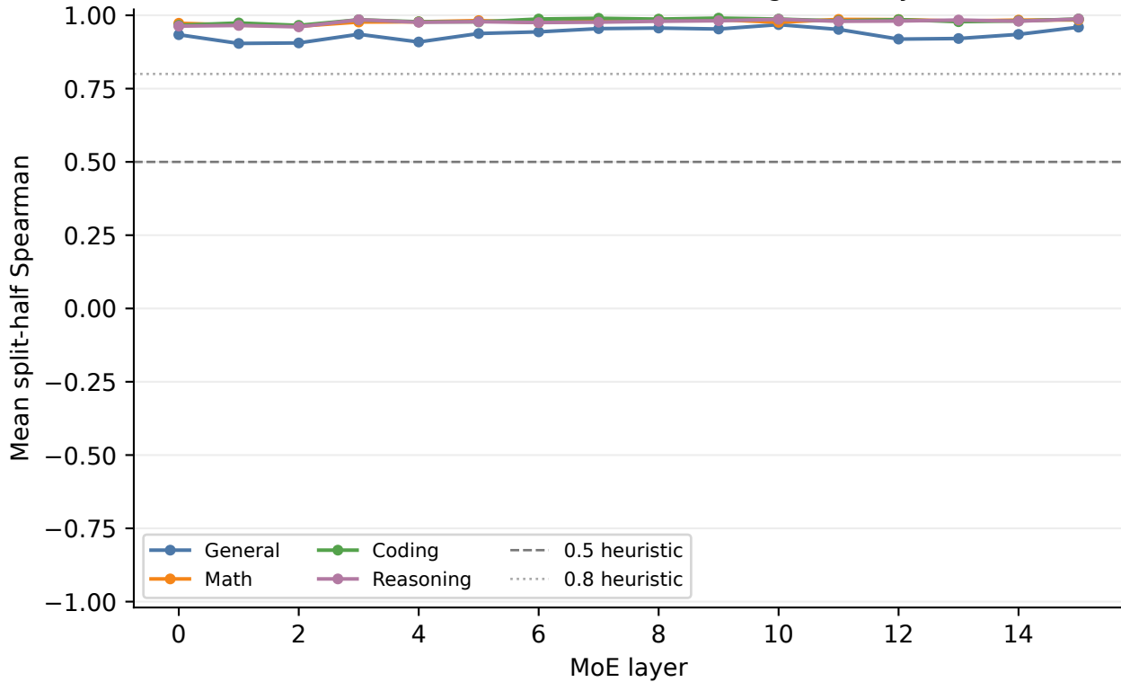
Within-domain functional-ranking reliability
