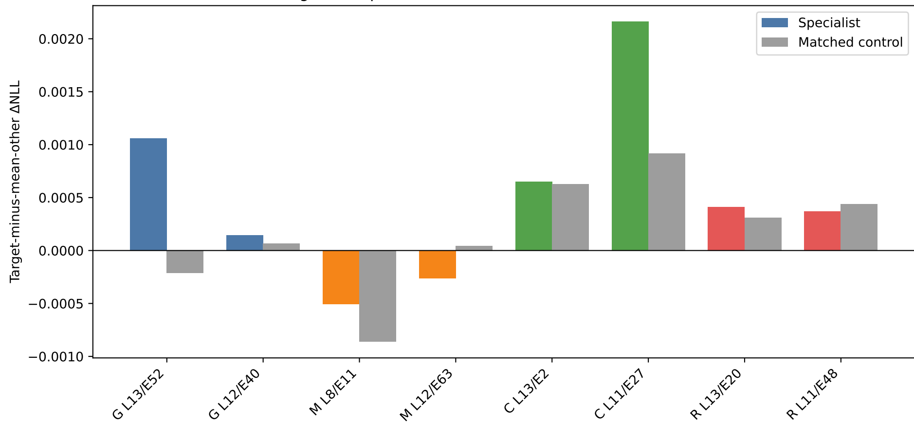
Figure 2: Specialist vs matched-control contrasts (4-bit)
