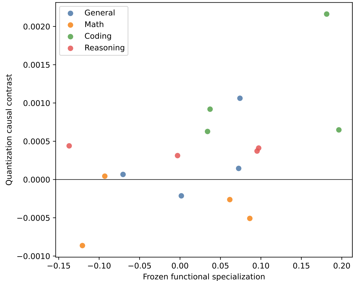
Figure 4: Functional vs quantization specificity (4-bit)
